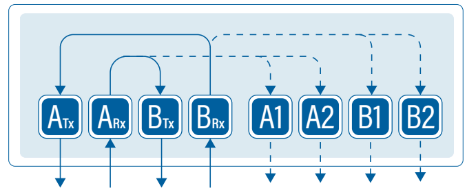
NETWORK PORTS
